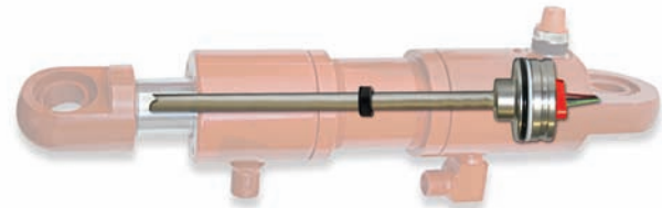
M-Series (Model MH) with digital output (sensor shown in cylinder application)
